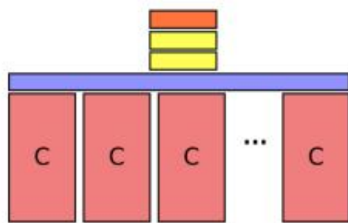
1) Conv Pooling
