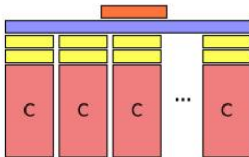
2) Late Pooling
