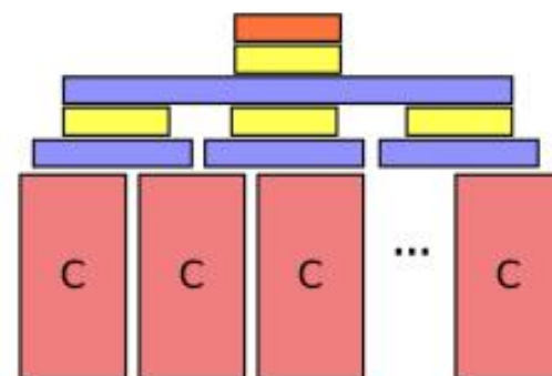
3) Slow Pooling
