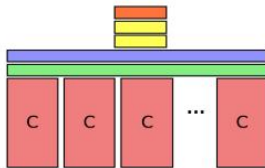
5) Time-domain convolution
